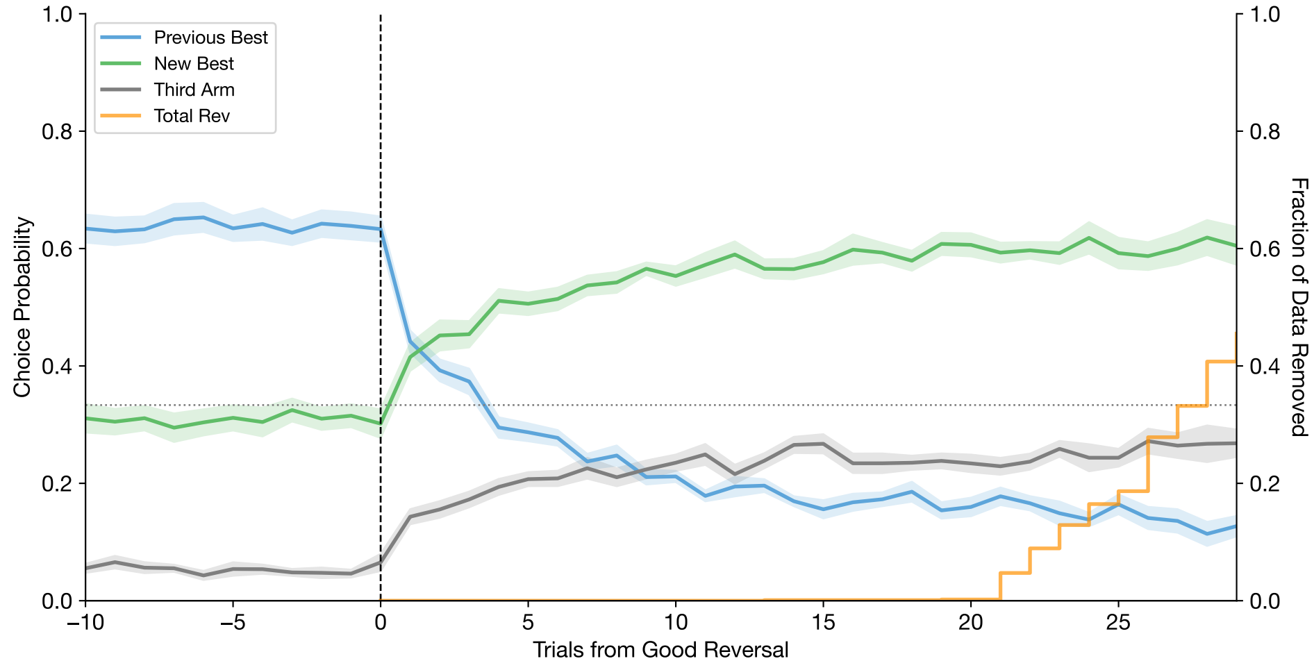
Reversal-Aligned Choices (mean \pm se across problems | n=6 subjects, n=928 reversals, n=18 problems)
